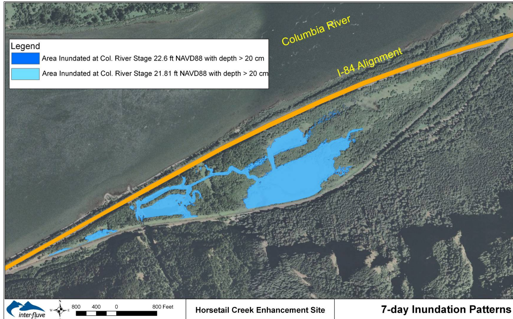
Figure 42. Inundation extents for areas with minimum 20 cm depth for the average of the annual maximum 7-day continuous stage over the period 1981-2010 (elevation 21.8) and the 2-year return period annual maximum 7-day continuous stage (elevation 22.6).
