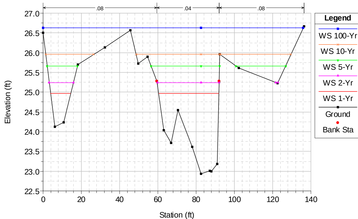
Figure 54. Simulated water surface elevations for the cross-section at Horsetail Creek RS 2499 in the alluvial fan reach. See Figure 49 for location.
