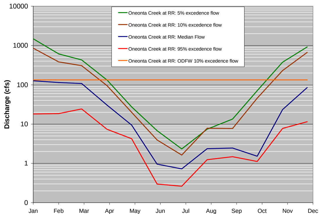
Figure 33. Fish passage flow duration statistics for Oneonta Creek at the UPRR bridge.
