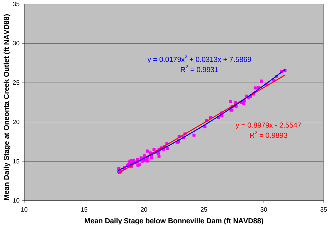
Figure 37. Correlation between daily mean river stage at the outlet of Oneonta Creek and below Bonneville Dam, over the period 04/01/10 – 09/29/10. Data was constrained to period when stage observations at Oneonta Creek outlet were greater than 13.5 ft NAVD88. Two alternate regressions of the data are shown.
