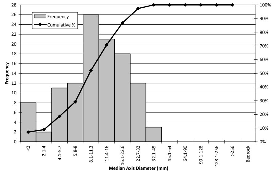
HT 1 Pebble Count Surficial Grain Size Analysis
