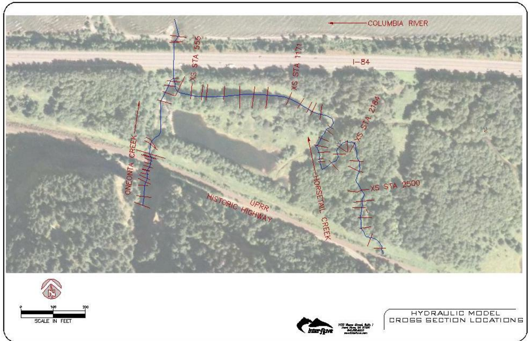
Figure 49. Hydraulic model cross section locations.
