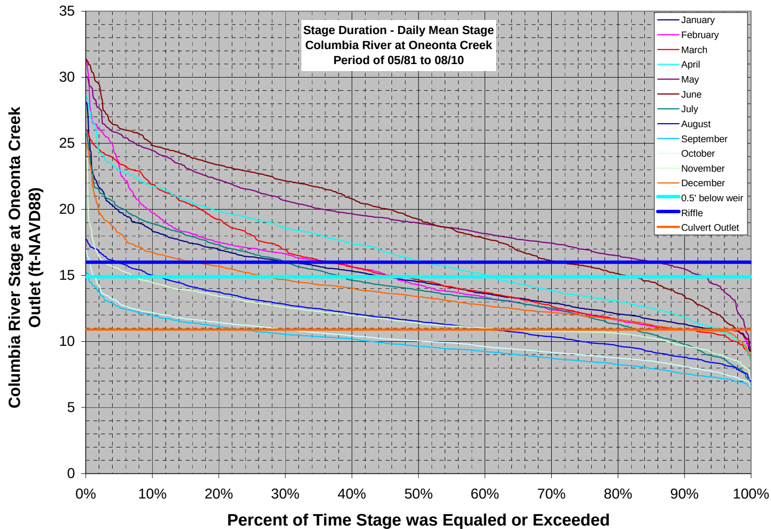
Figure 40. Mean daily stage duration curves for Columbia River at outlet of Oneonta Creek, estimated over the e period 1981-2010. Cyan horizontal line labeled 0.5' below weir corresponds to the water surface elevation for which the hydraulic drop over the concrete weir upstream of the Oneonta Creek culvert would match fish passage criteria for juvenile salmonids. Blue horizontal line corresponds to the elevation of the crest of the first riffle in Horsetail Creek upstream of the Oneonta Creek culvert. Orange horizontal line corresponds to invert elevation at outlet of Oneonta Creek culvert.
