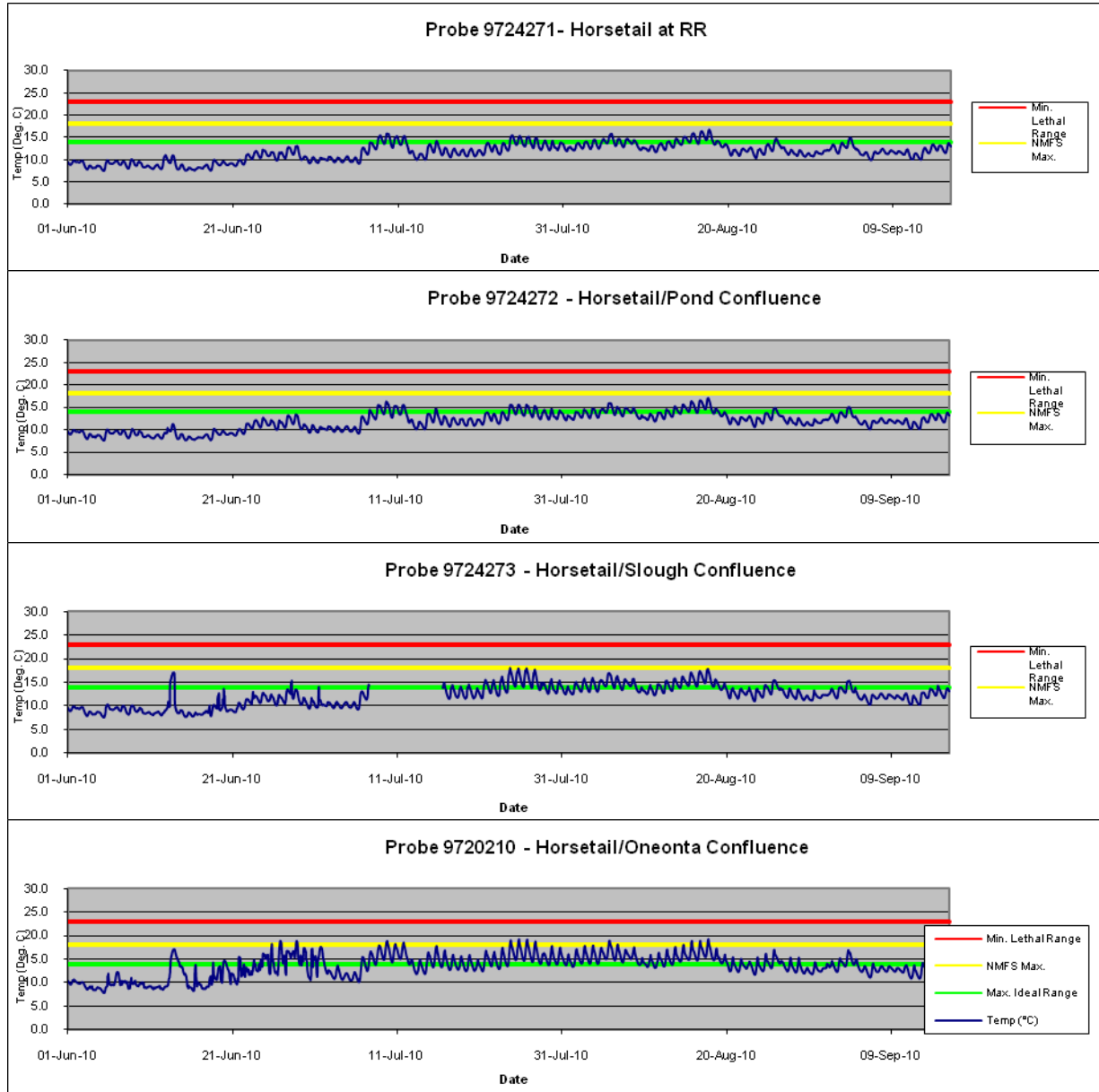
Figure 47 a-d. Thermal profiles for Horsetail Creek monitoring stations. Refer to Section 1.1.1 for detail regarding the threshold values presented in the graphs.
