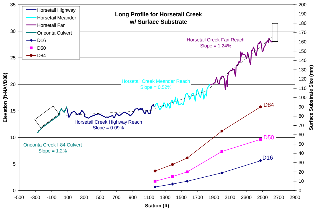
Figure 22. Comparison of surface substrate size to channel slope in Horsetail Creek.
