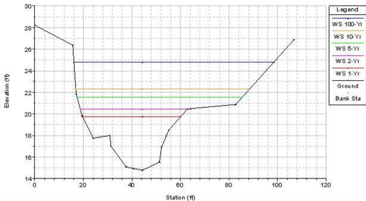
Figure 52. Simulated water surface elevations for the cross-section at Horsetail Creek RS 1171 in the highway reach. See Figure 49 for location.
