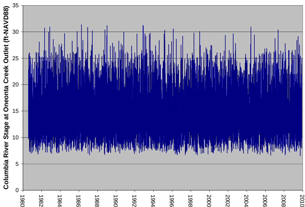
Figure 38. Time series of estimated Columbia River daily mean stage at outlet of Oneonta Creek, over the period 1980 – 2010.
