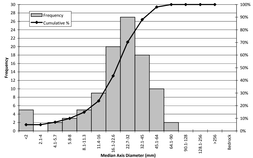
HT 3 Pebble Count Surficial Grain Size Analysis
