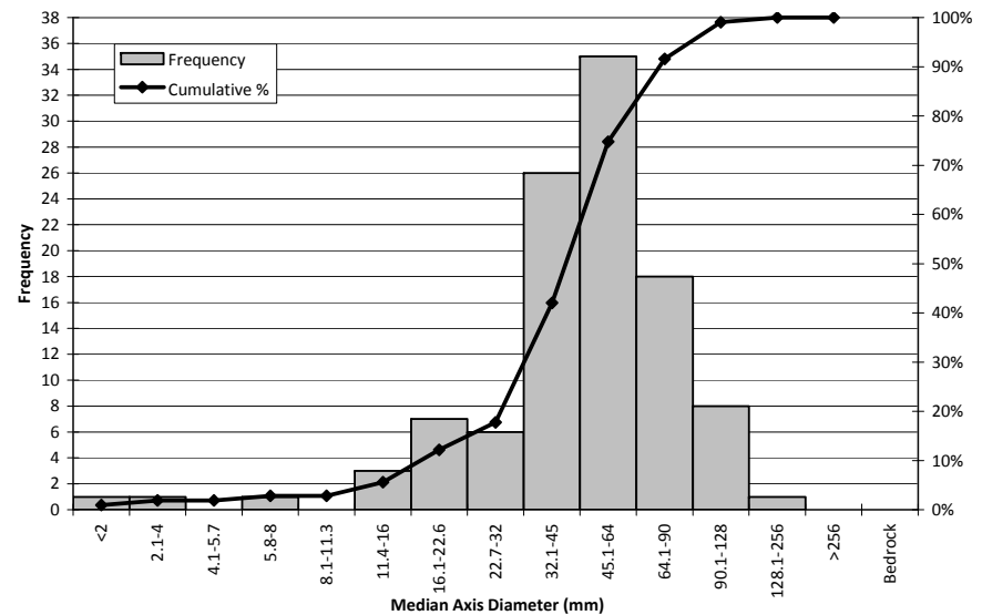
HT 4 Pebble Count Surficial Grain Size Analysis
