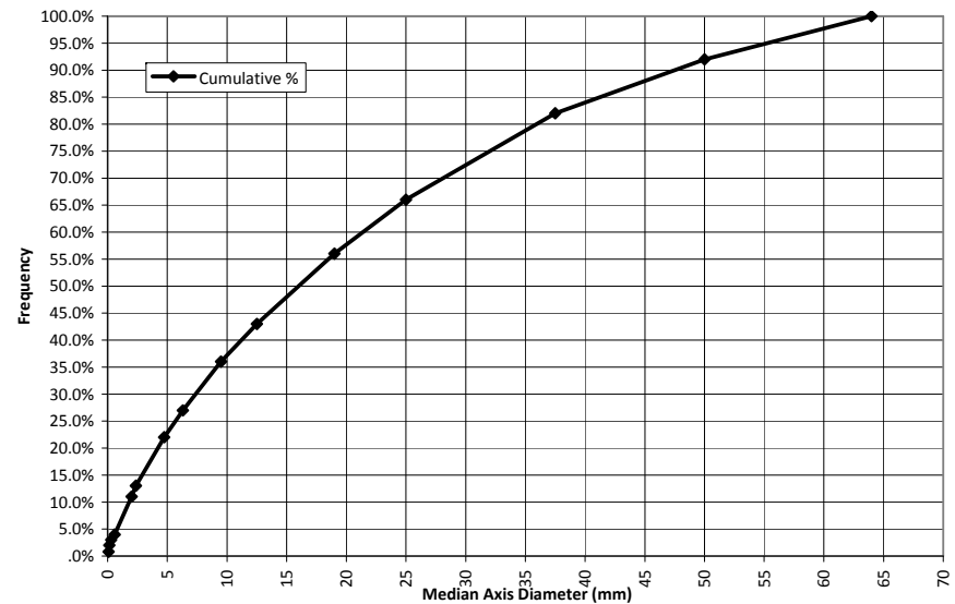
HT 3 Subsurface Grain Size Analysis
