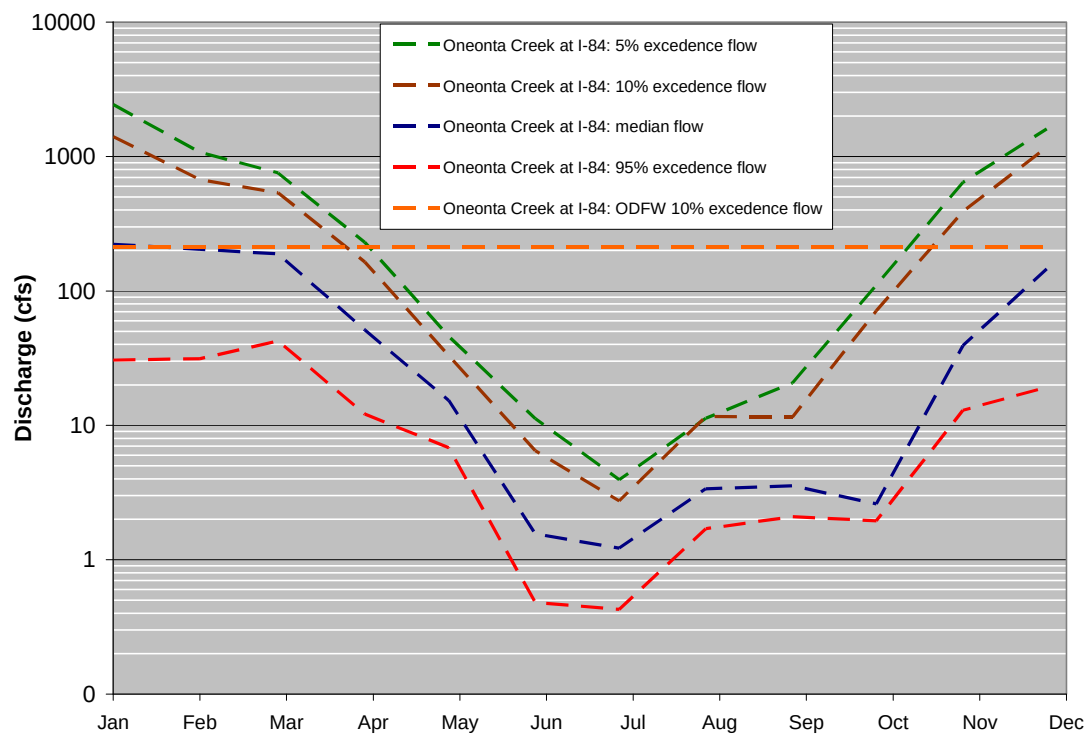
Figure 34. Fish passage flow duration statistics for Oneonta Creek at the I-84 crossing.
