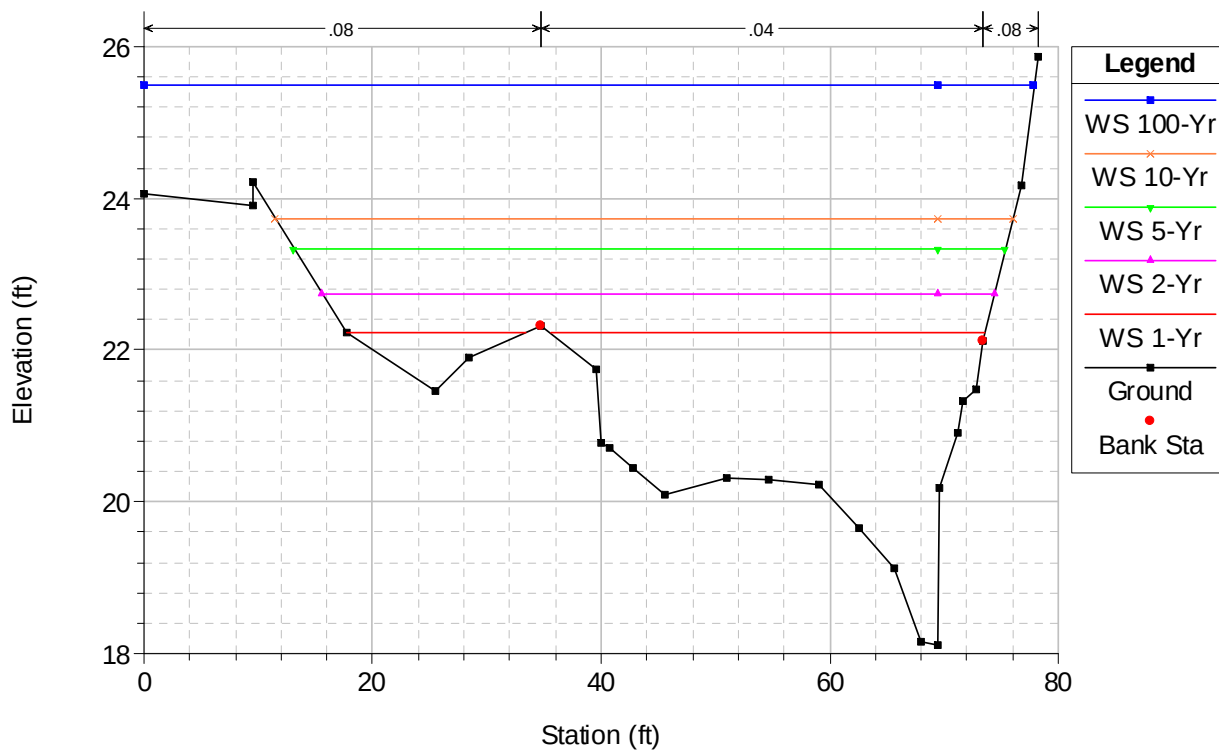
Figure 53. Simulated water surface elevations for the cross-section at Horsetail Creek RS 2184 in the meander reach. See Figure 49 for location.
