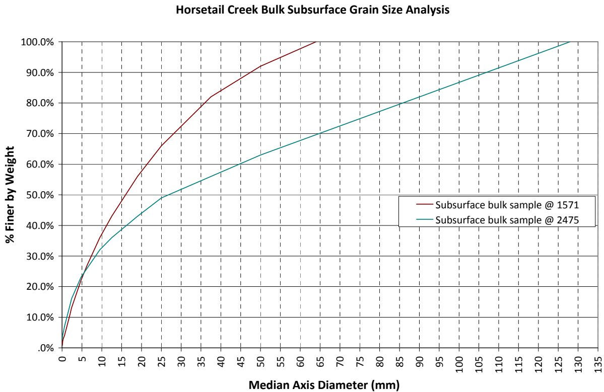
Figure 23. Subsurface bulk sediment data results.
