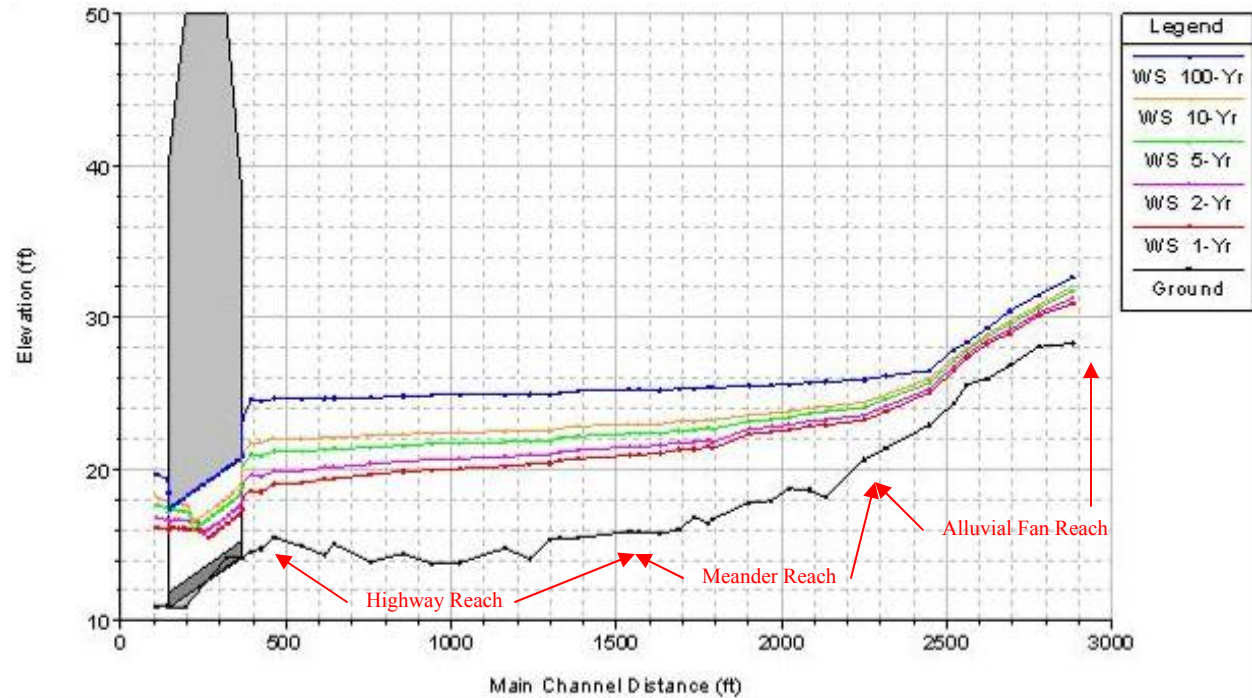
Figure 50. Simulated water surface profiles for existing conditions at a range of high flow events.
