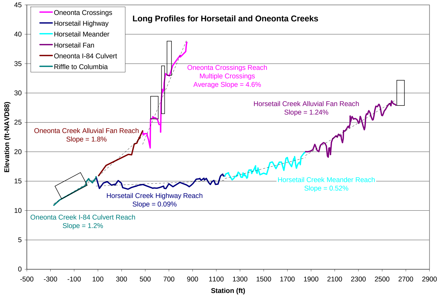
Figure 20. Longitudinal thalweg profiles for Horsetail and Oneonta Creeks.
