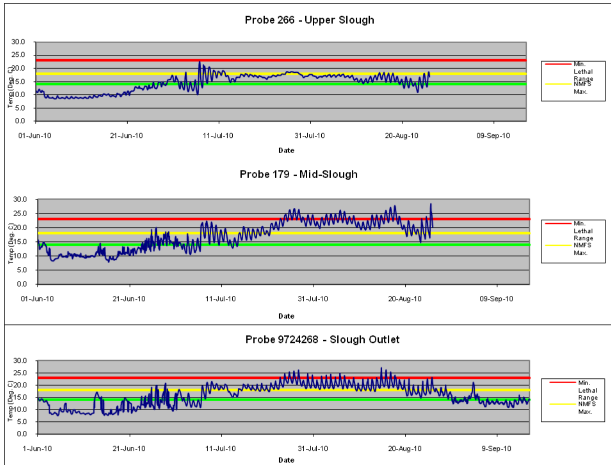
Figure 48 a-c. Thermal profiles for Horsetail Creek monitoring stations. Refer to Section 3.3.1.3.1 for detail regarding the threshold values presented in the graph.
