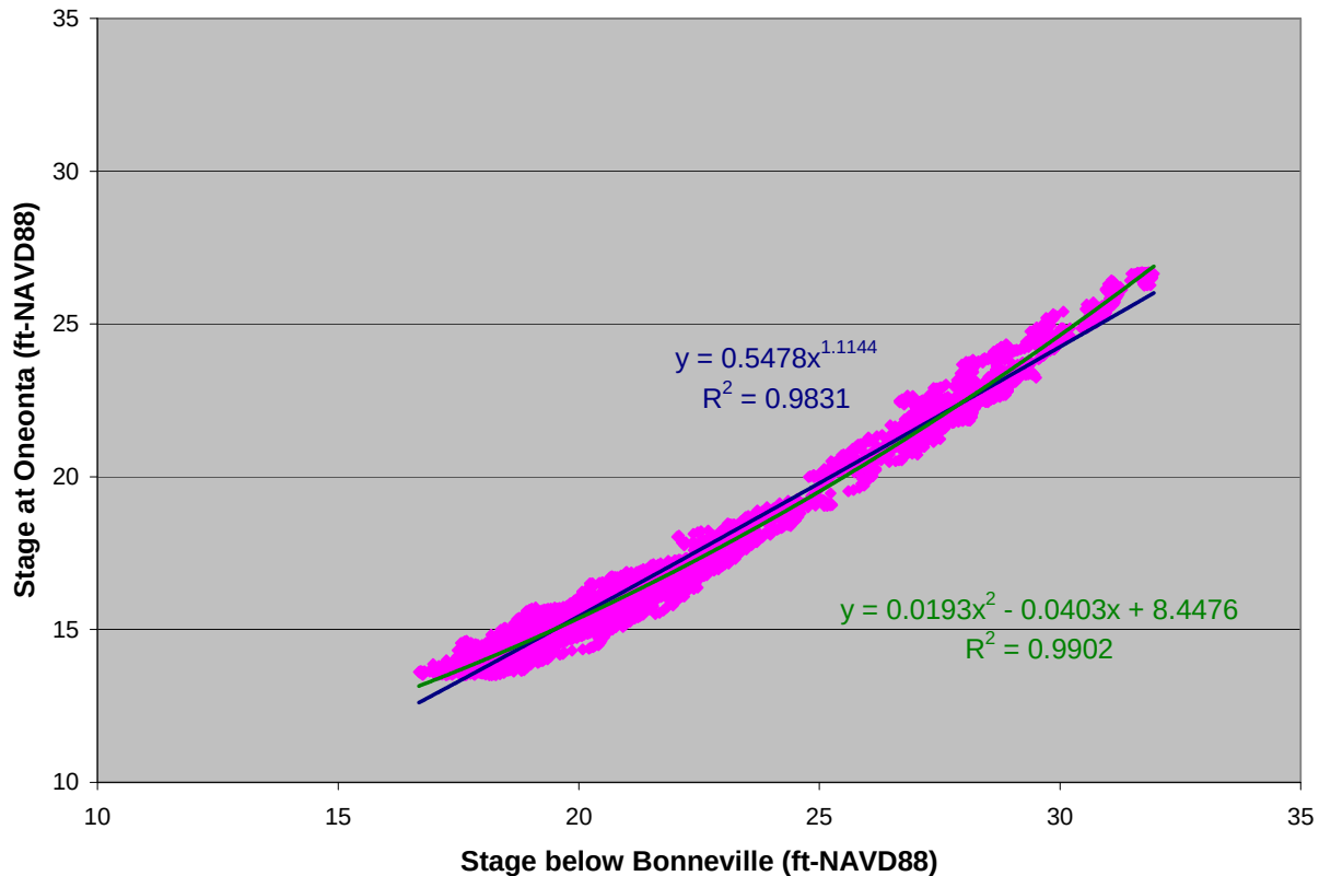
Figure 36. Correlation between river stage at the outlet of Oneonta Creek and below Bonneville Dam, using 15 min data over the period 04/01/10 – 09/29/10, assuming a 2-hour lag between the two locations. Data was constrained to period when stage observations at Oneonta Creek outlet were greater than 13.5 ft NAVD88. Two alternate regressions of the data are shown.
