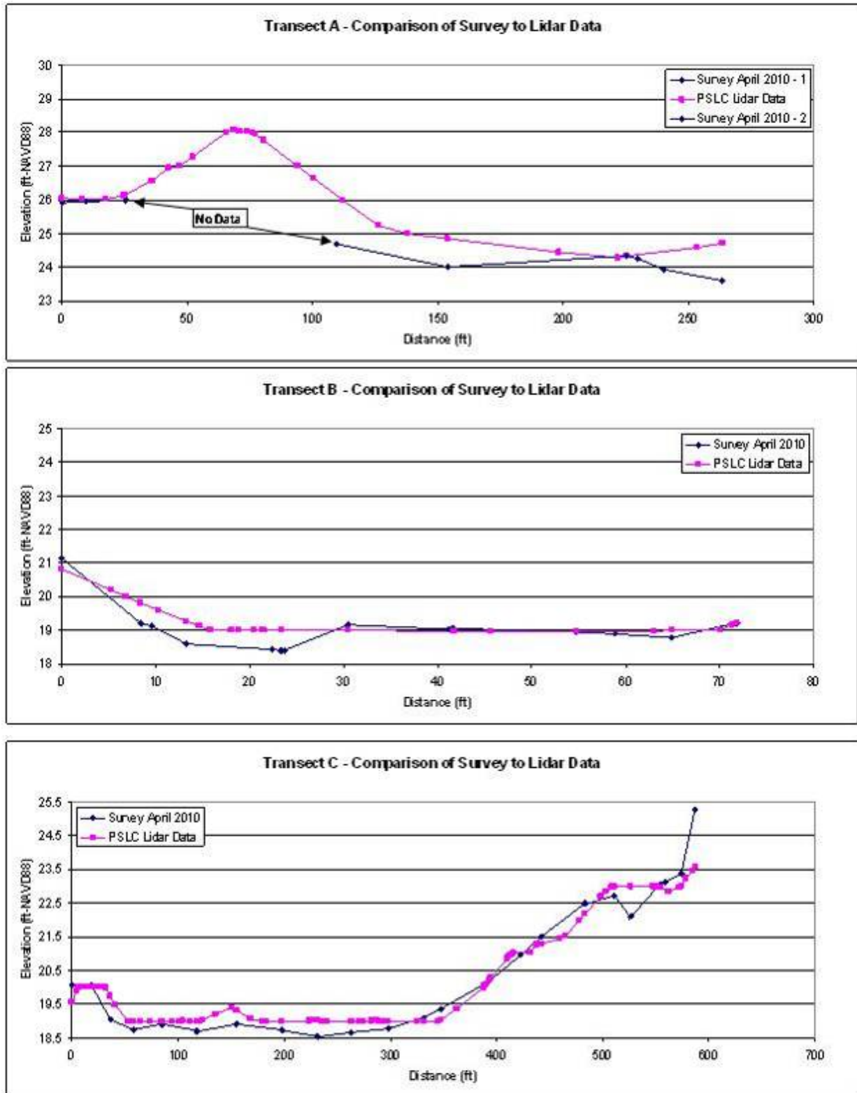
Figure 18 a-c. Transects A-C comparing surveyed ground elevations to PSLC lidar data.
