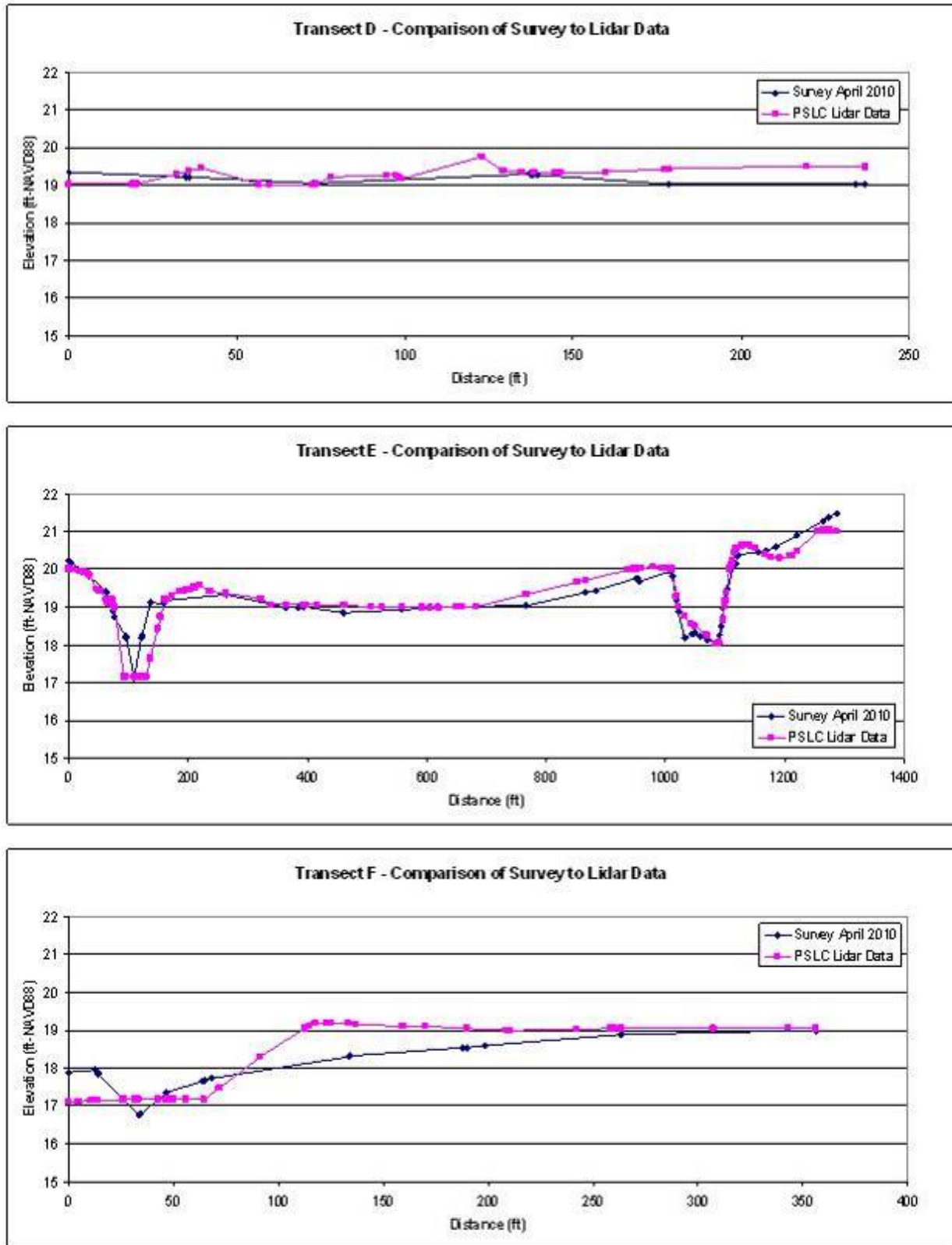
Figure 19 a-c. Transects D-F comparing surveyed ground elevations to PSLC lidar data.
