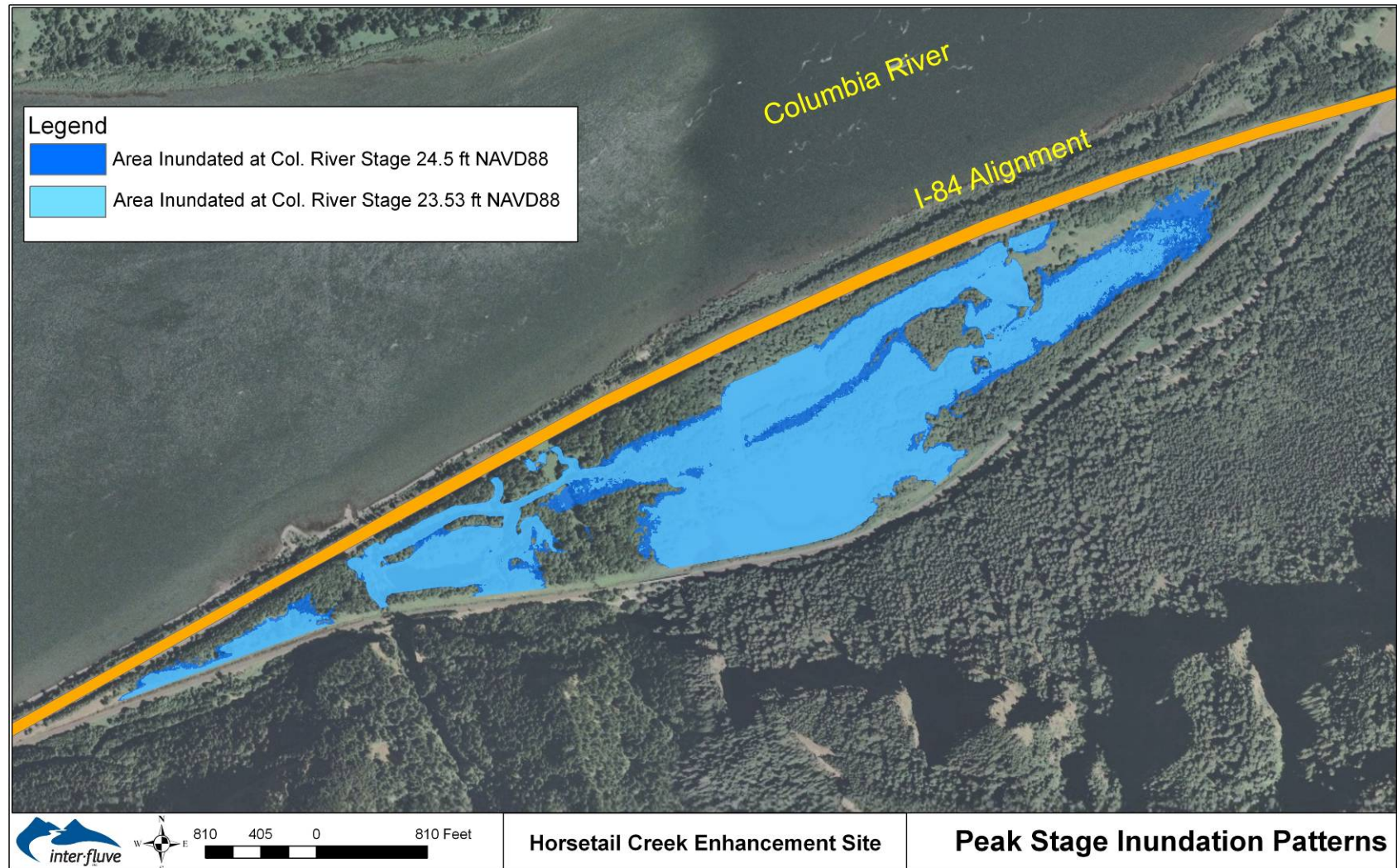
Figure 41. Inundation extents for the average of the annual peak stage over the period 1981-2010 (elevation 23.5) and the 2-year return period peak stage, based on data over the period 1981-2010 (elevation 24.5).
