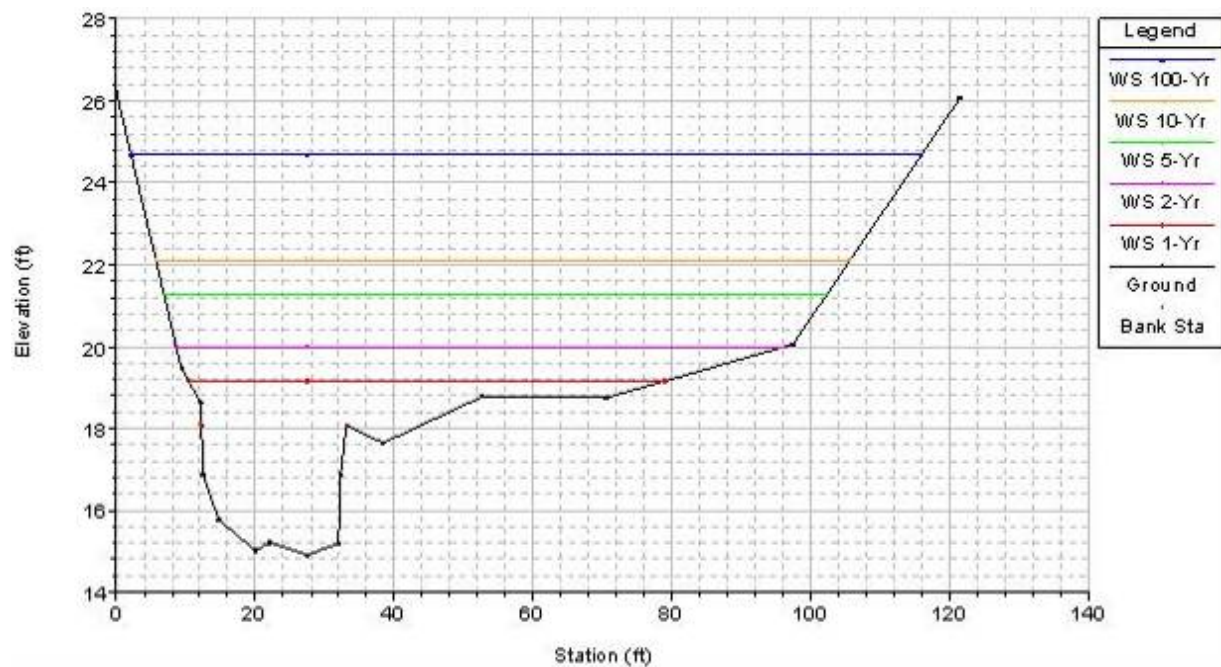
Figure 51. Simulated water surface elevations for the cross-section at Horsetail Creek RS 555 in the highway reach. See Figure 49 for location.
