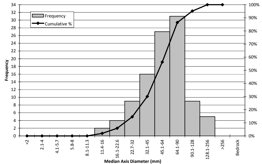
HT 5 Pebble Count Surficial Grain Size Analysis
