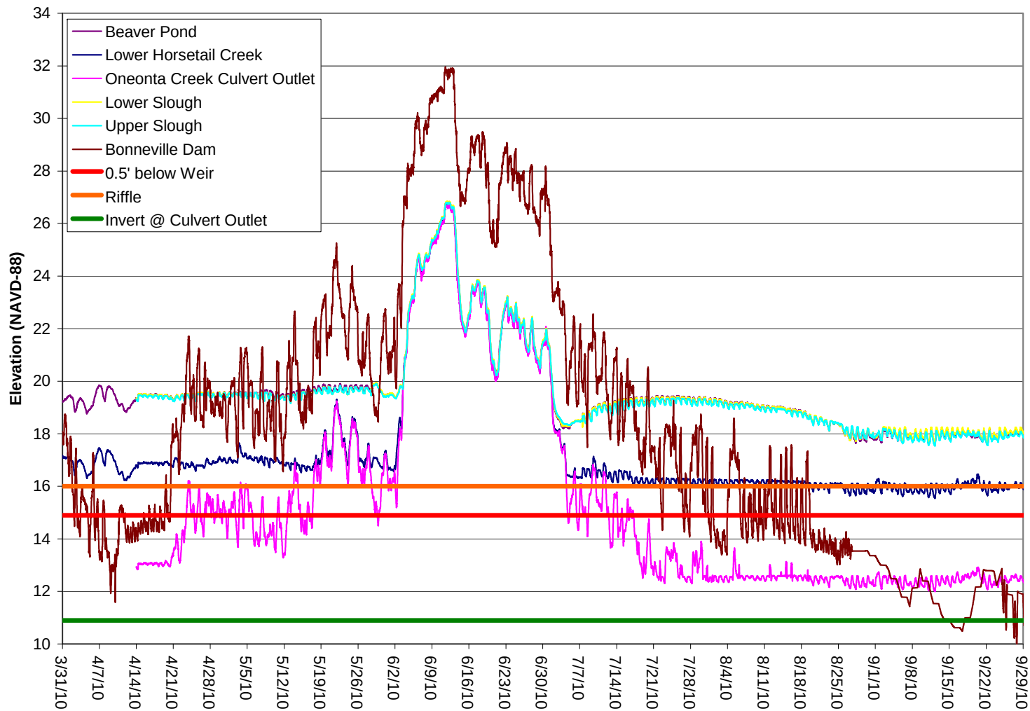
Figure 35. Measured stage at Horsetail Creek site with locally deployed pressure transducers 04/01/10 to 09/29/10. Bonneville Dam data from USGS gage 14128870 Columbia River below Bonneville Dam. See footnotes to Table 8 for additional explanations of data. Red horizontal line labeled 0.5' below weir corresponds to the water surface elevation for which the hydraulic drop over the concrete weir upstream of the Oneonta Creek culvert would match fish passage criteria for juvenile salmonids. Orange horizontal line corresponds to the elevation of the crest of the first riffle in Horsetail Creek upstream of the Oneonta Creek culvert. Green horizontal line corresponds to invert elevation at outlet of Oneonta Creek culvert.
