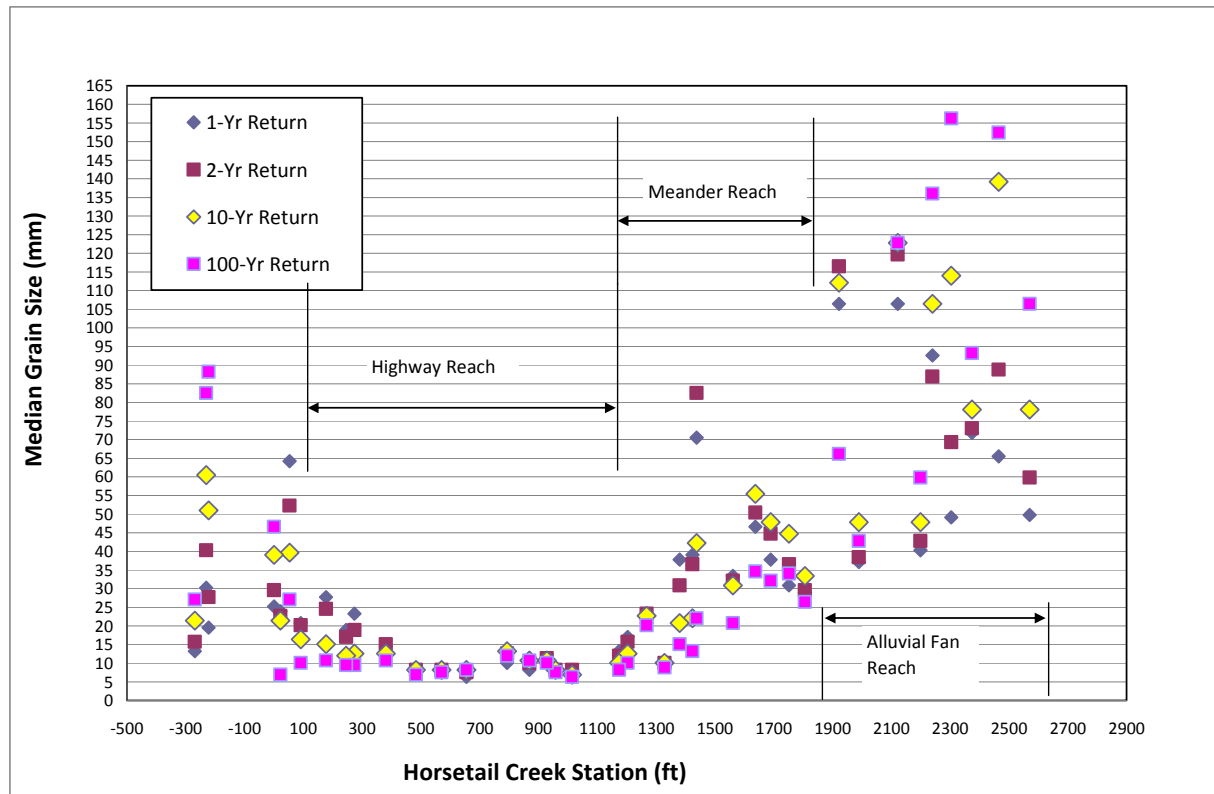
Figure 55. Channel competence results for Horsetail Creek under existing conditions. River Station 0 is at the confluence of Horsetail and Oneonta Creeks in this figure. Add 379 feet to the stationing in the figure to convert to the hydraulic model stationing discussed above, which includes the Oneonta Creek culvert.
